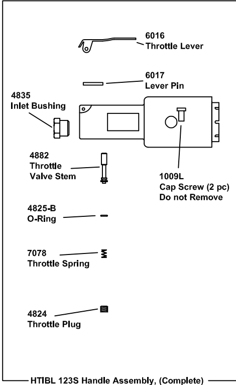
HTIBL 123S Handle Assembly, (Complete)
